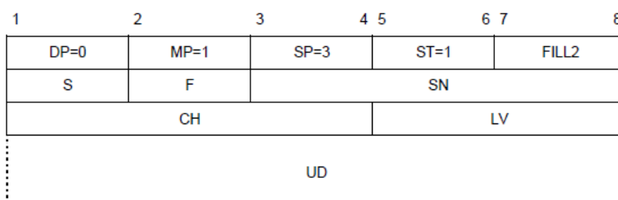
Figure 5-12. INTERRUPT packet
