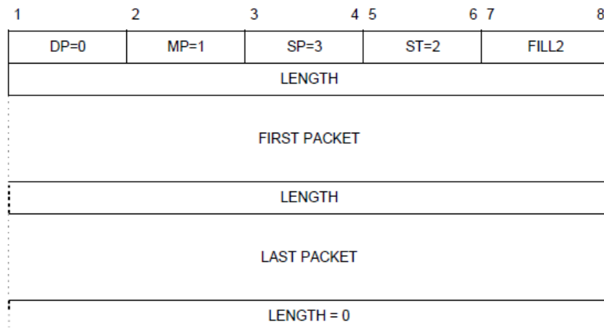
Figure 5-20. MULTIPLEX packet
