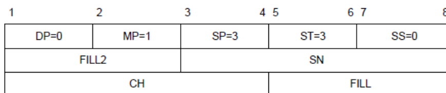
Figure 5-13. INTERRUPT CONFIRMATION packet
