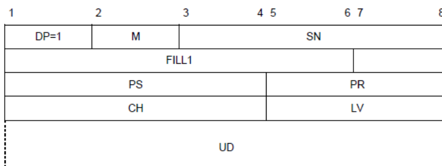
Figure 5-11. DATA packet
