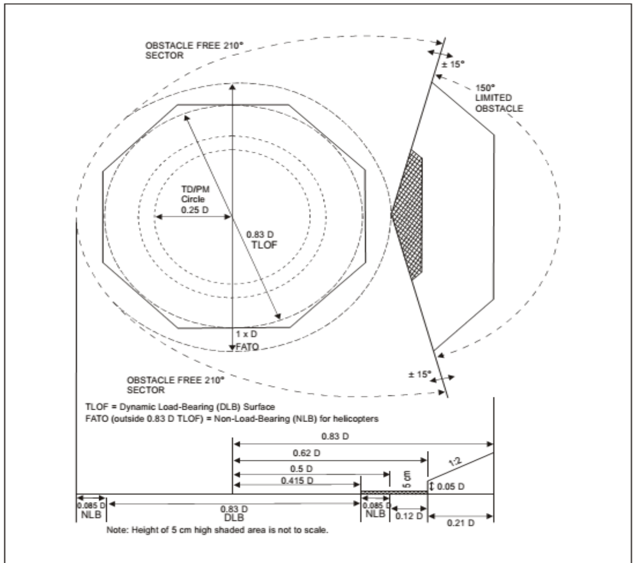
Figure 4-9. Helideck obstacle limitation sectors and surfaces for
