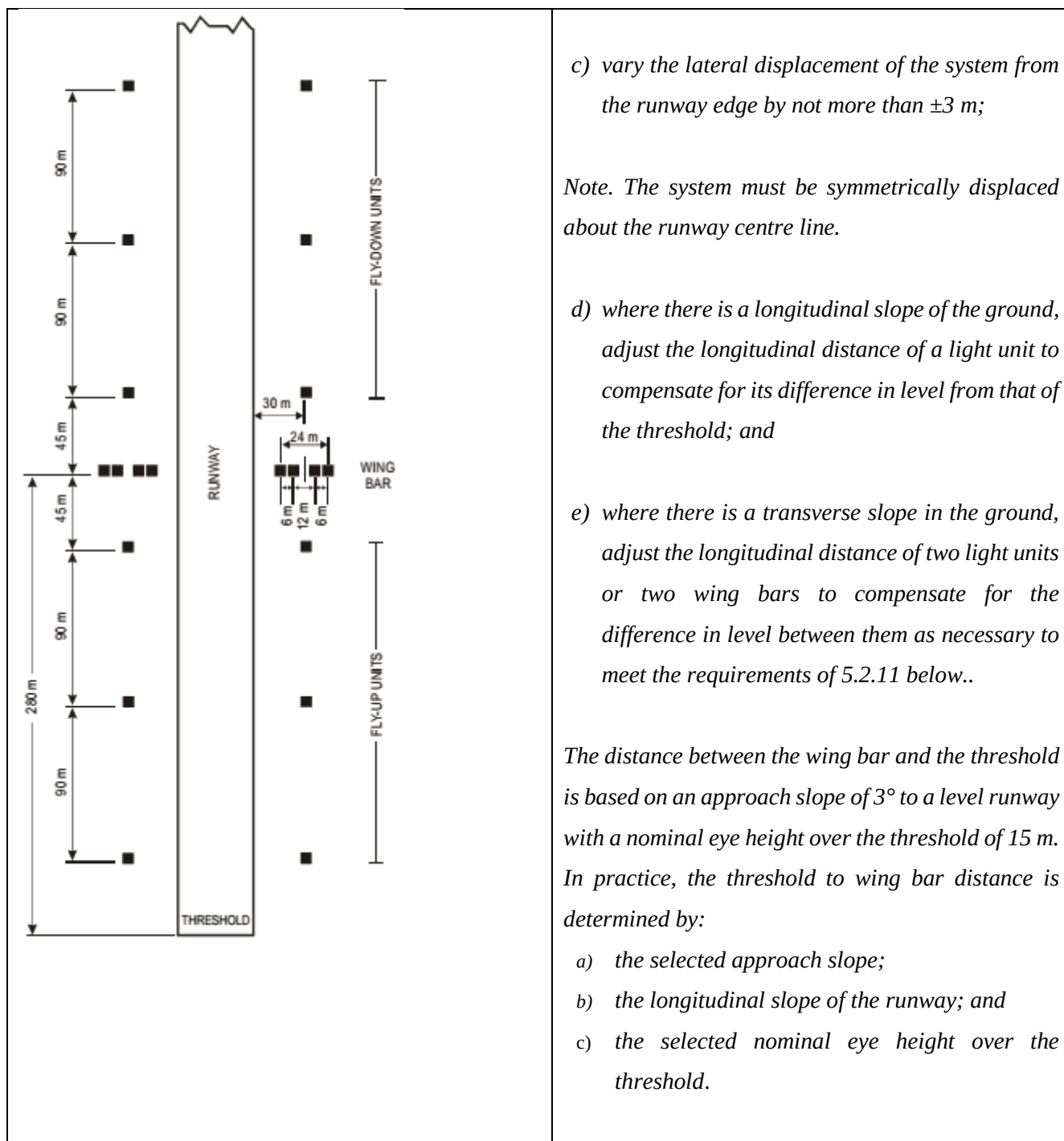
Figure 12. 25: Siting of light units for T-VASIS (Edit figure)
