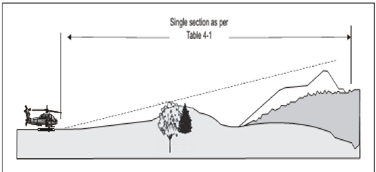
Figure 4-6. Approach and take-off climb surfaces with different slope design categories
